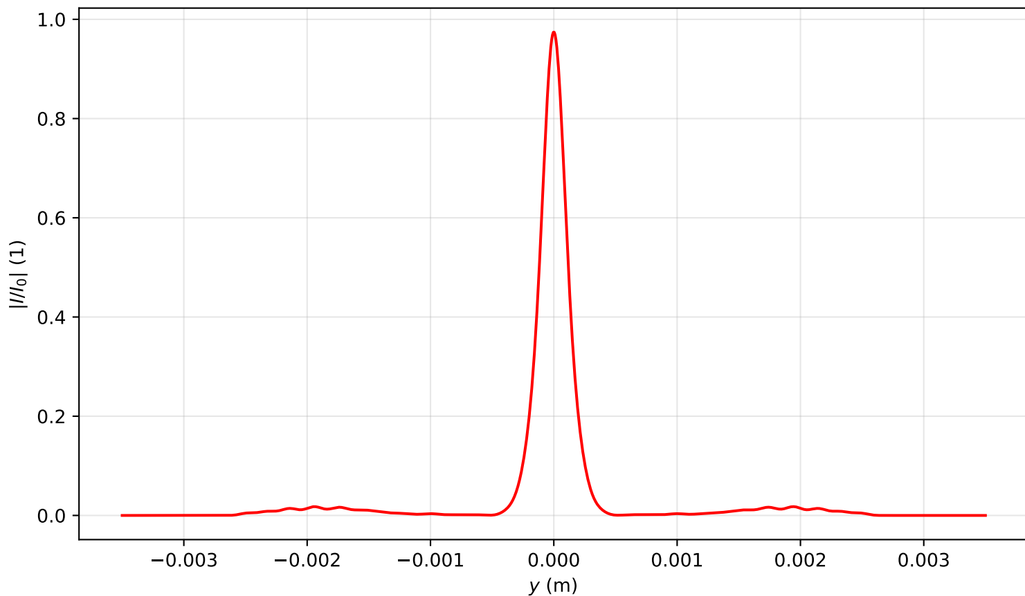
Intensity profile I(x=0, y, z=1.433)/I_0 , \text{Pin}=6.0\text{Pcr} , artificial time
